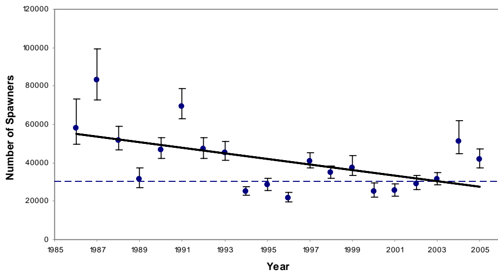
Fig. 8. Annual lake-wide population estimates of spawning-phase sea lampreys in Lake Ontario during 1986–2005 with trend line (solid line), 95% confidence intervals (vertical lines) and target level (dashed line).
