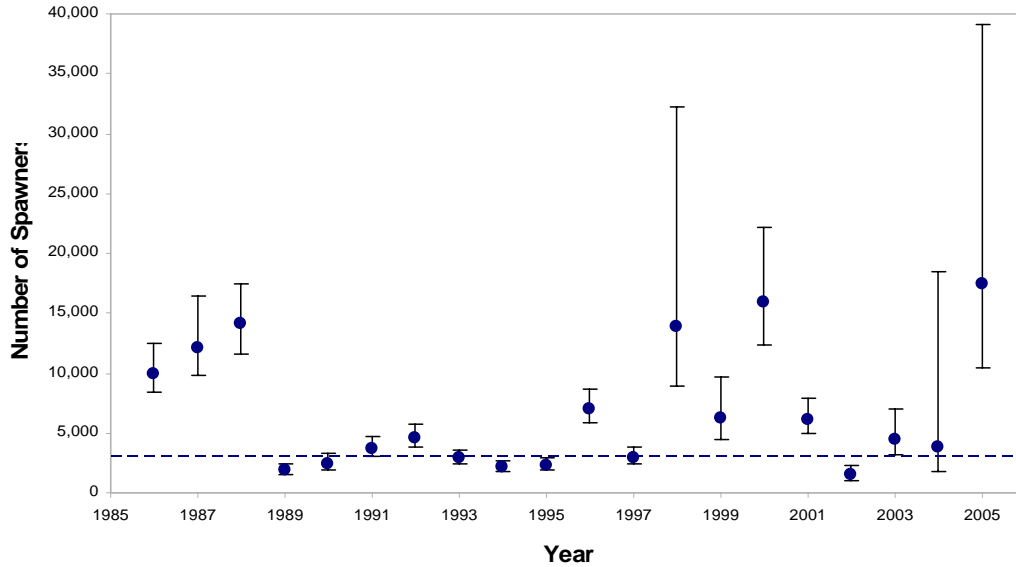
Fig. 7. Annual lake-wide population estimates of spawning-phase sea lampreys in Lake Erie during 1986–2005 with 95% confidence intervals (vertical lines) and target level (dashed line).
