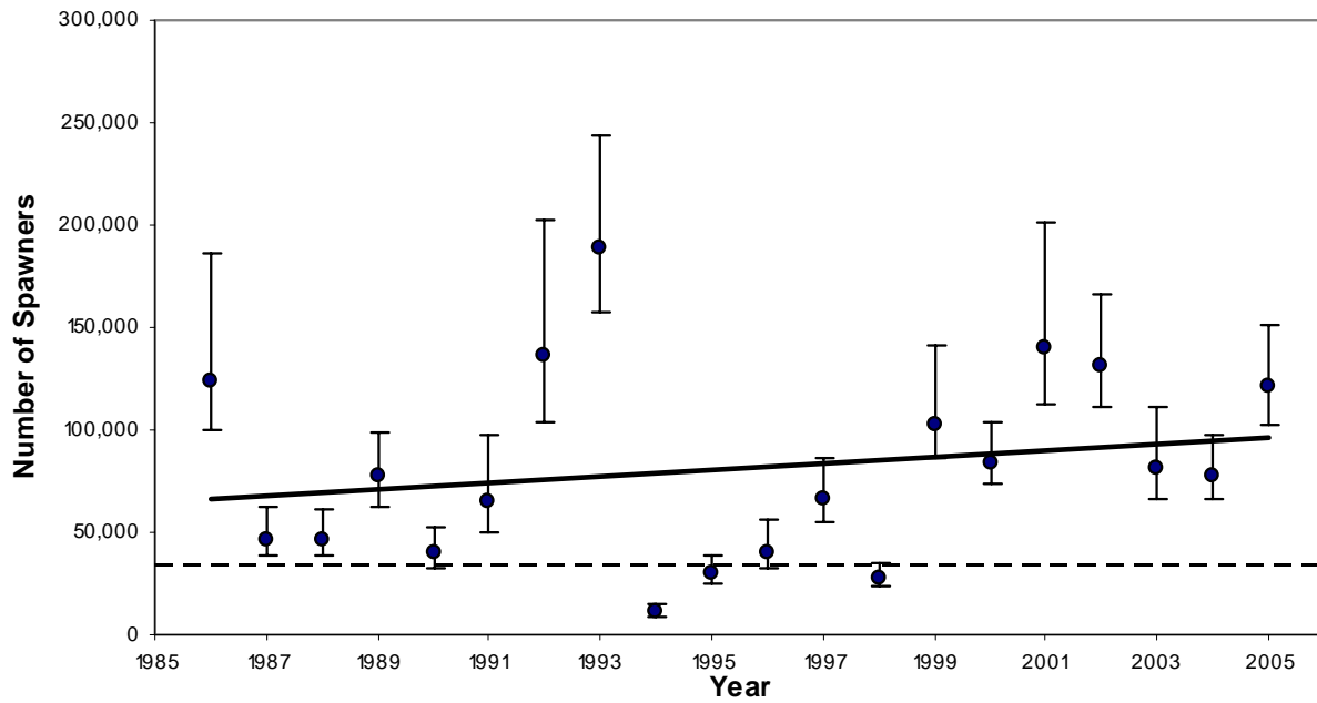
Fig. 4. Annual lake-wide population estimates of spawning-phase sea lampreys in Lake Superior during 1986 – 2005 with 95% confidence intervals (vertical lines) and target level (dashed line).
