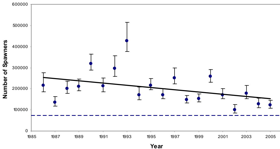
Fig. 6. Annual lake-wide population estimates of spawning-phase sea lampreys in Lake Huron during 1986–2005 with 95% confidence intervals (vertical lines) and target level (dashed line).
