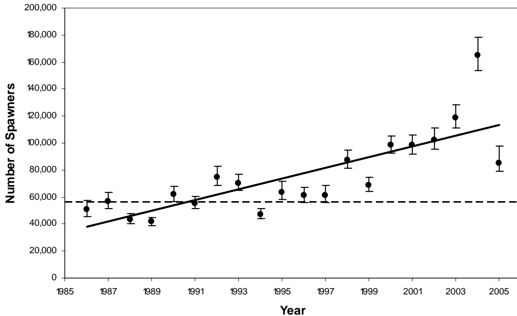
Fig. 5. Annual lake-wide population estimates of spawning-phase sea lampreys in Lake Michigan during 1986 – 2005 with trend line (solid line), 95% confidence intervals (vertical lines), and target level (dashed line).
